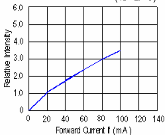
FIG. 2 Relative Intensity vs. Forward Current ( T_a = 25^\circ\text{C} )
