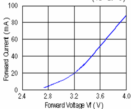
FIG. 1 Forward Current vs. Forward Voltage ( T_a = 25^\circ\text{C} )
