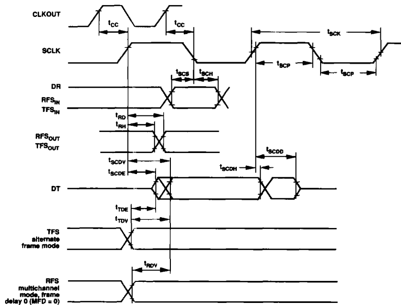
Figure 20. Serial Ports
