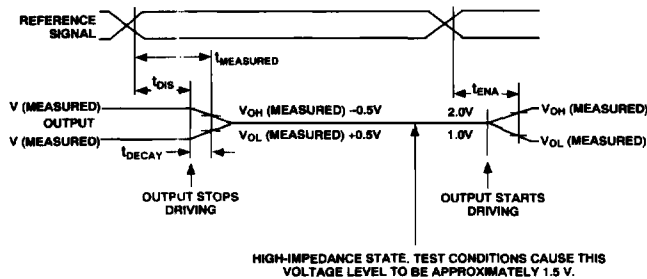
Figure 31. Output Enable/Disable
