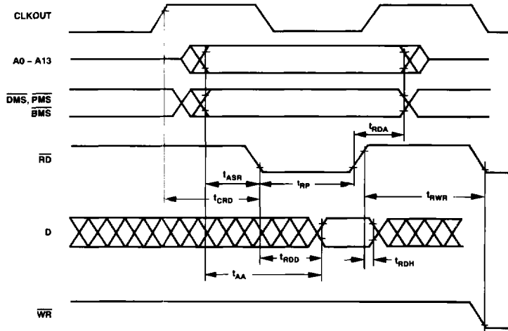
Figure 18. Memory Read
