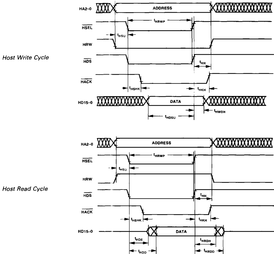
Figure 22. Host Interface Port (HMD1 = 0, HMD0 = 1)
