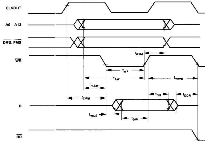
Figure 19. Memory Write
