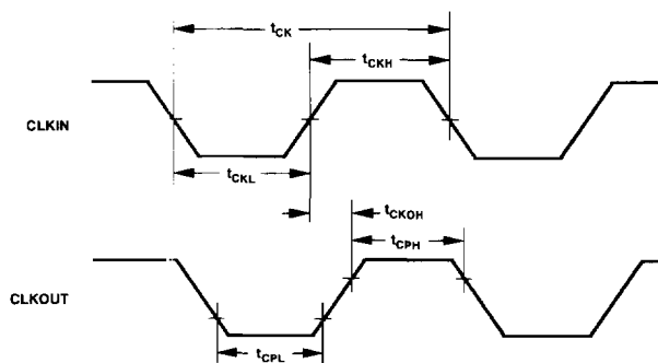
Figure 15. Clock Signals
