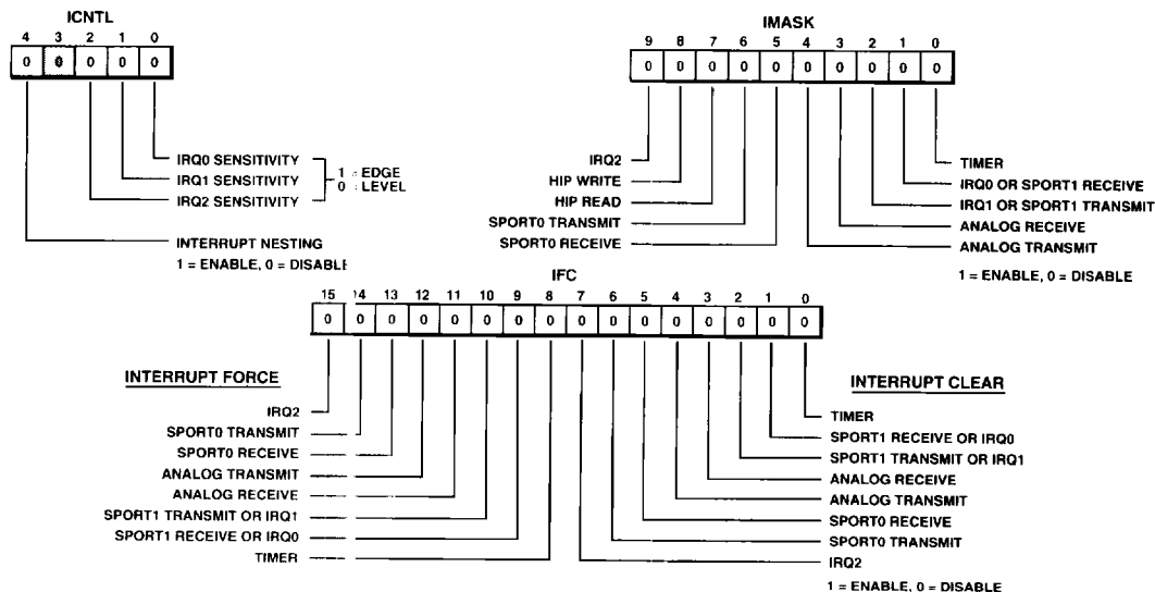
Figure 2. Interrupt Registers
