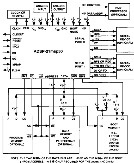
Figure 3. ADSP-21msp5xA Basic System Configuration
