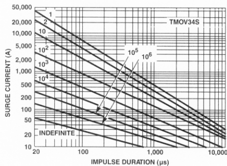
FIGURE 6. SURGE CURRENT RATING CURVES FOR TMOV34S
