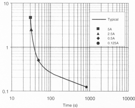
* Figure 4: Typical time to open circuit under UL1449 Abnormal Overvoltage Limited Current Test
