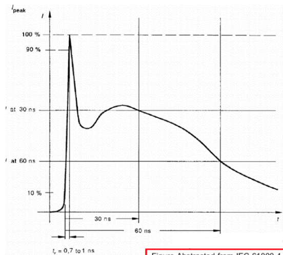
Figure Abstracted from IEC 61000-4-2 © IEC 1995, 1998, 2000
