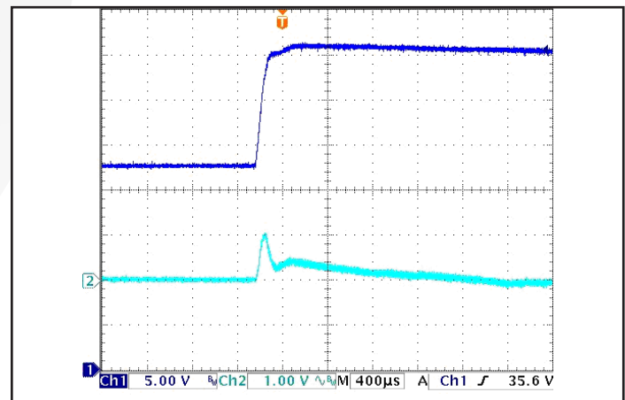
Figure 12: Output voltage response to step-change in input voltage (250V/ms). Load cap: 330 µF electrolytic output capacitance. Ch 1: V_{in} (5V/div), Ch 2: V_{out} (1V/div).
