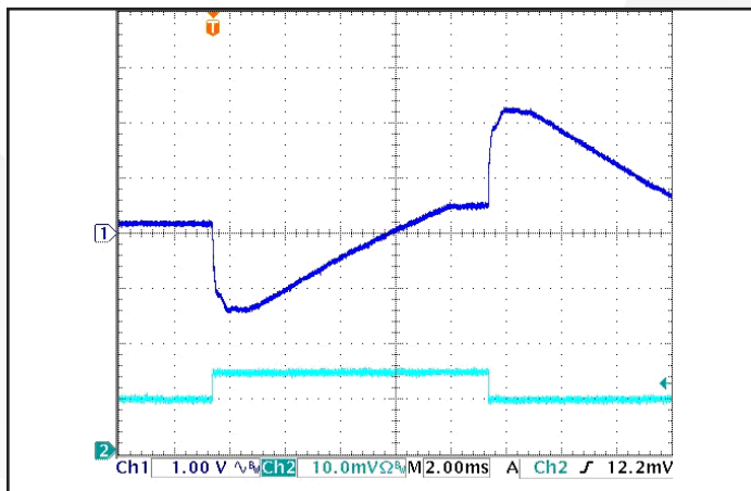
Figure 11: Output voltage response to step-change in load current (50%-75%-50% of I_{out(max)} ; dI/dt = 5 A/\mu s ). Load cap: 1 µF ceramic and 100 µF electrolytic capacitors. Ch 1: V_{out} (1V/div), Ch 2: I_{out} (5A/div).
