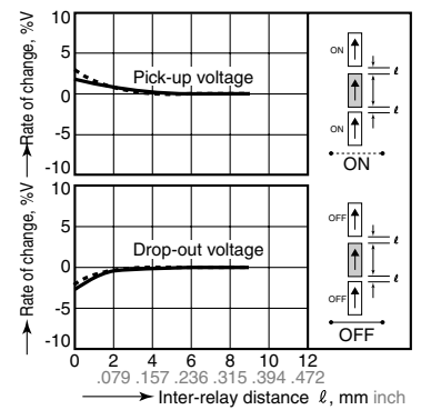
9-(2). Influence of adjacent mounting Tested sample: AGN20012, 6 pcs.
