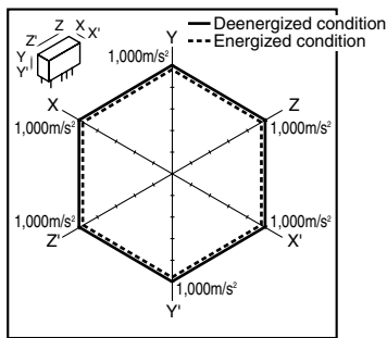
8. Malfunctional shock Tested sample: AGN2004H
