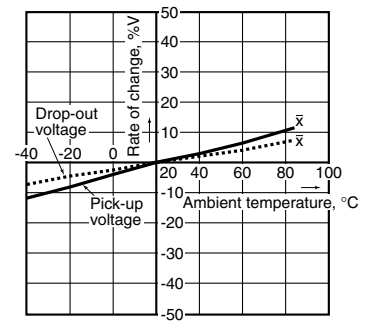
7. Ambient temperature characteristics Tested sample: AGN2004H, 6 pcs.
