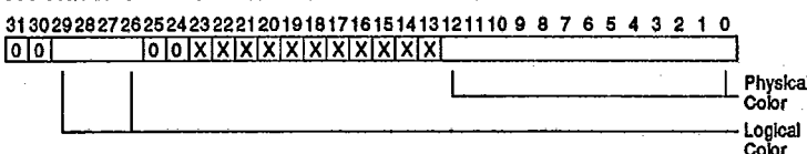
FIGURE 4. VIDEO PHYSICAL COLOR FORMAT
