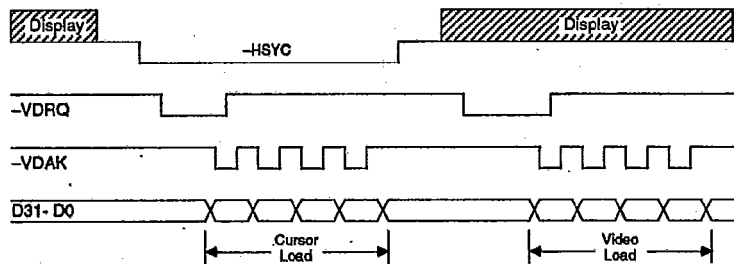
FIGURE 29. VIDEO DMA OVERLAPPING -HSYC PULSE
