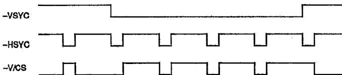
FIGURE 39. INTERLACE DISPLAY TIMING GENERATION
