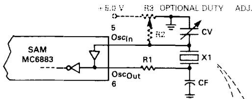
FIGURE 9 — CRYSTAL OSCILLATOR
