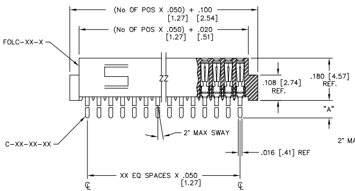
SECT "A-A"
