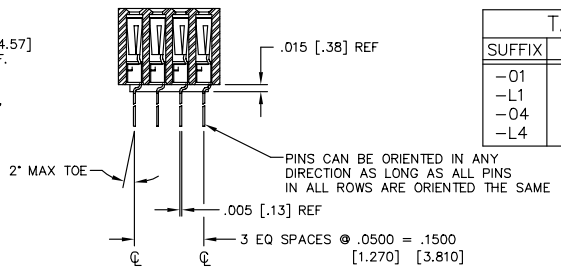
SECT "B-B"
