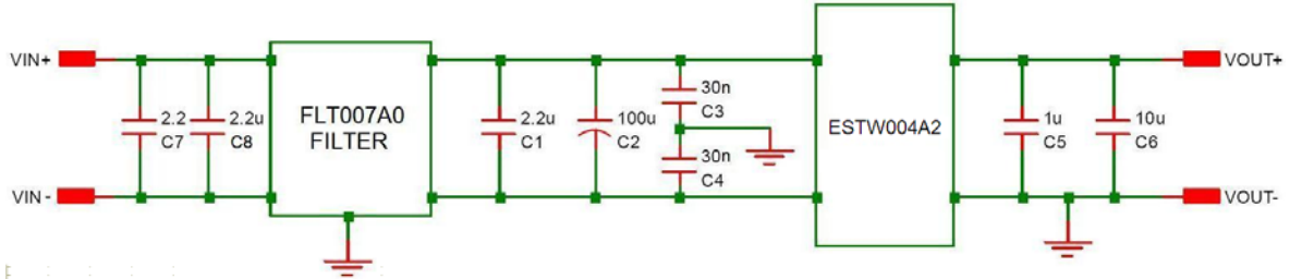
Figure 23. EMC Considerations
