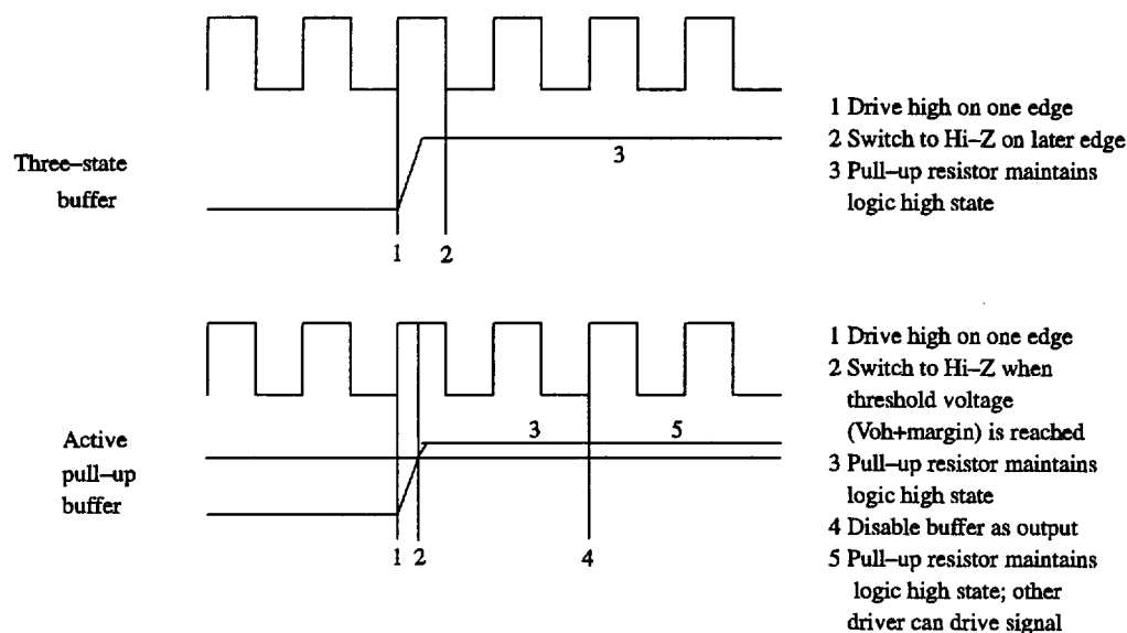
Figure 6 : Three-State Buffers and Active Pull-Up Buffers
