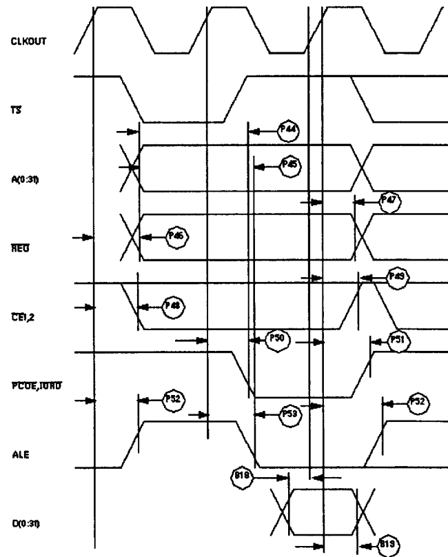
Figure 29 : PCMCIA access cycles Timing External Bus Read
