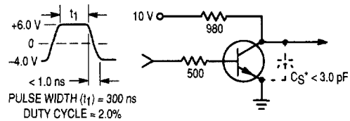
Figure 3. Storage Test Circuit
