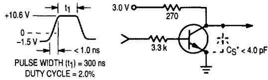
Figure 1. t_{on} Circuit
