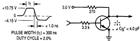
Figure 2. t_{off} Circuit
