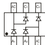
CDBV6-54BR-G Marking: KLB
