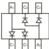
CDBV6-54AD-G* Marking: KL6
