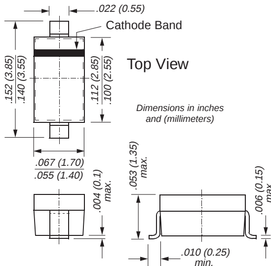
SOD-123
