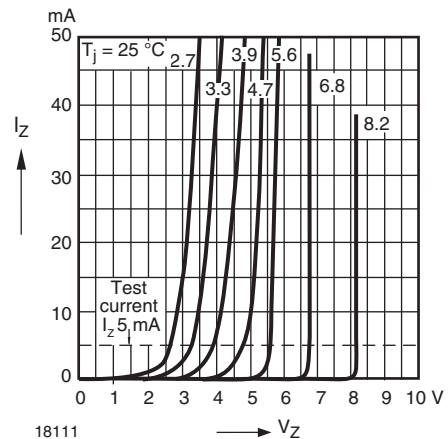
Figure 12. Breakdown Characteristics
