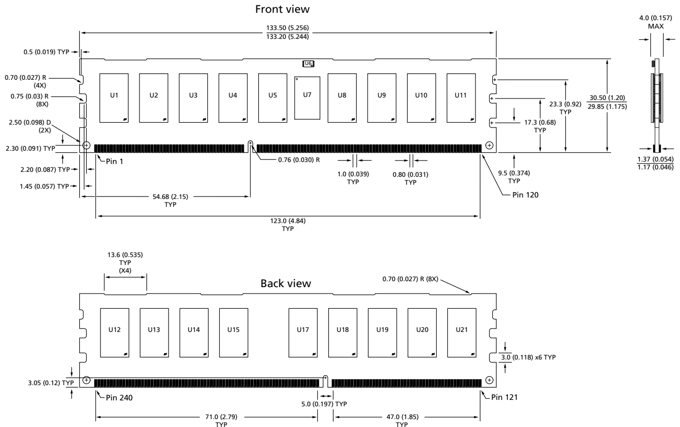
Figure 5: 240-Pin DDR3 RDIMM
