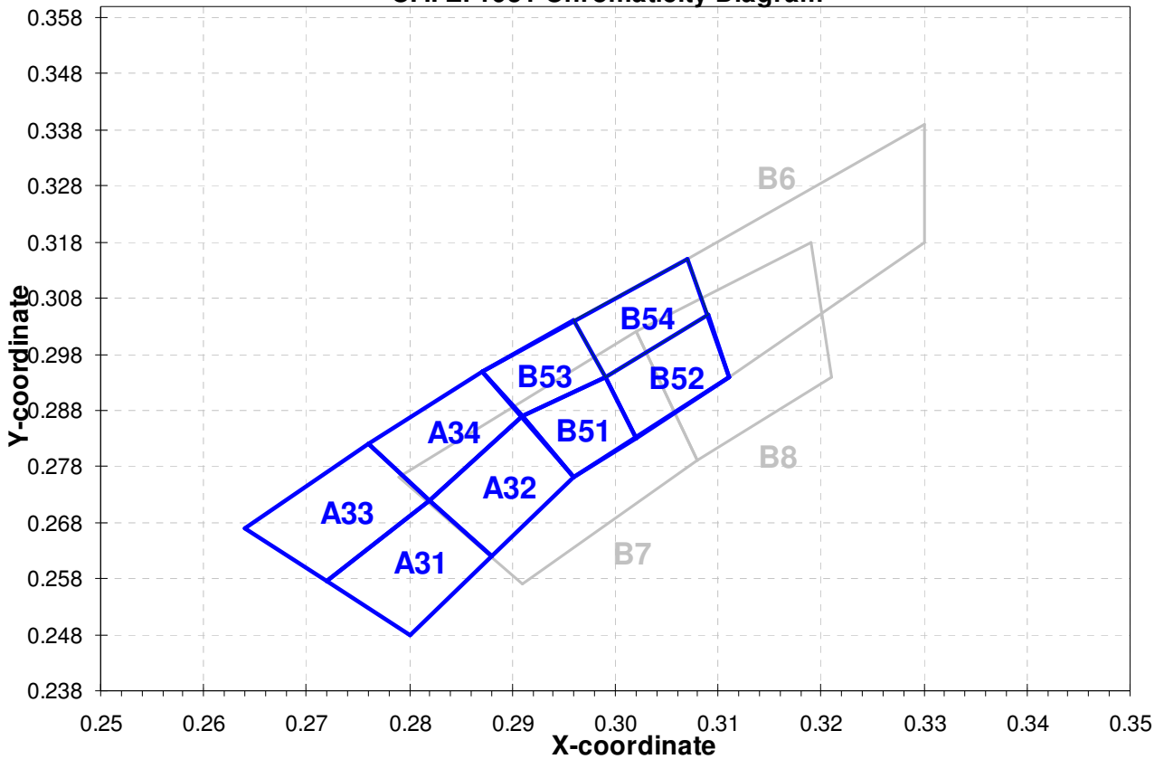
C. I. E. 1931 Chromaticity Diagram
