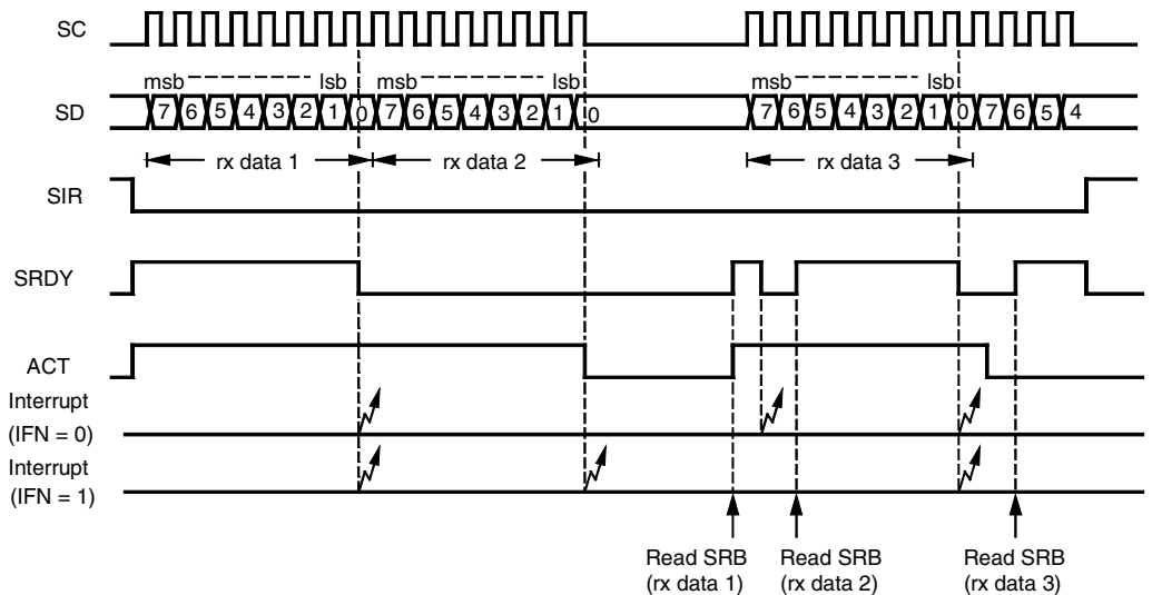
Figure 46. Example of 8-bit Synchronous Receive Operation
