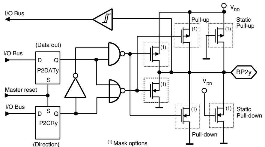
Figure 22. Bi-directional Port 2
