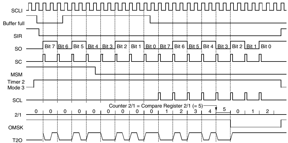
Figure 57. Bi-phase Modulation 2
