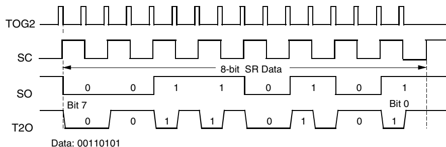
Figure 39. Bi-phase Modulation
