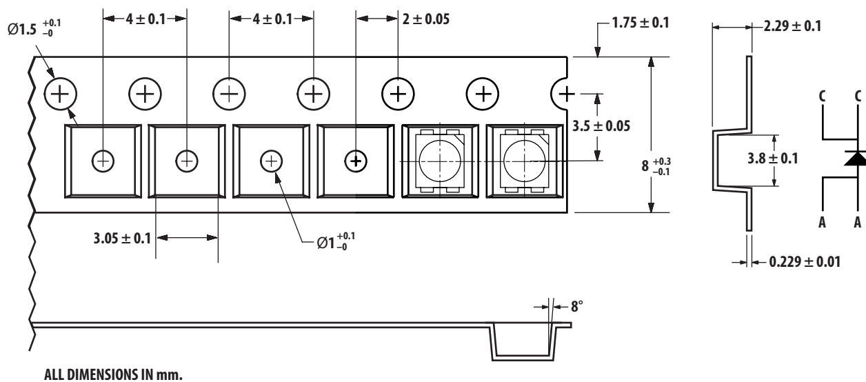
Figure 14. Tape Dimensions
