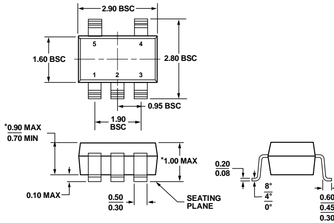
*COMPLIANT TO JEDEC STANDARDS MO-193-AB WITH THE EXCEPTION OF PACKAGE HEIGHT AND THICKNESS. Figure 37. 5-Lead Thin Small Outline Transistor Package [TSOT] (UJ-5) Dimensions shown in millimeters
