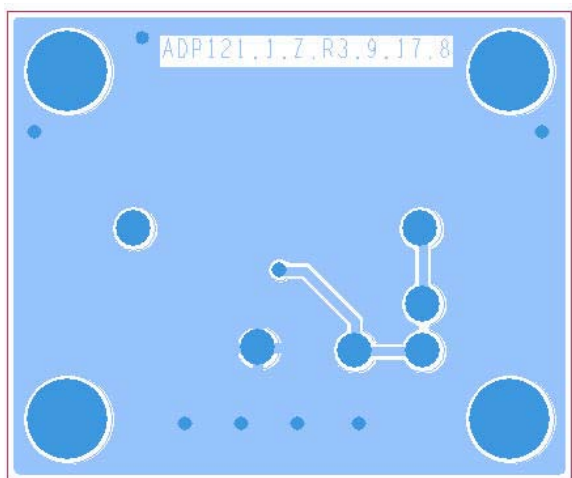
Figure 50. Example of WLCSP PCB Layout—Bottom Side
