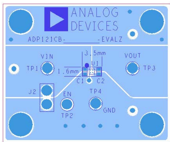
Figure 49. Example of WLCSP PCB Layout—Top Side
