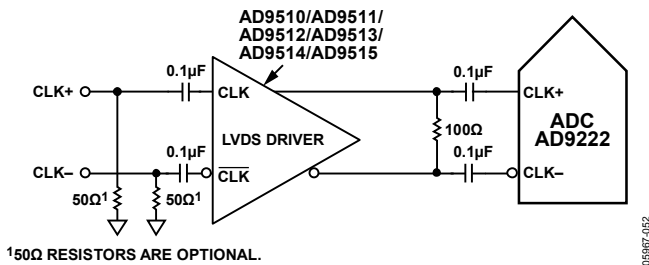
Figure 65. Differential LVDS Sample Clock
