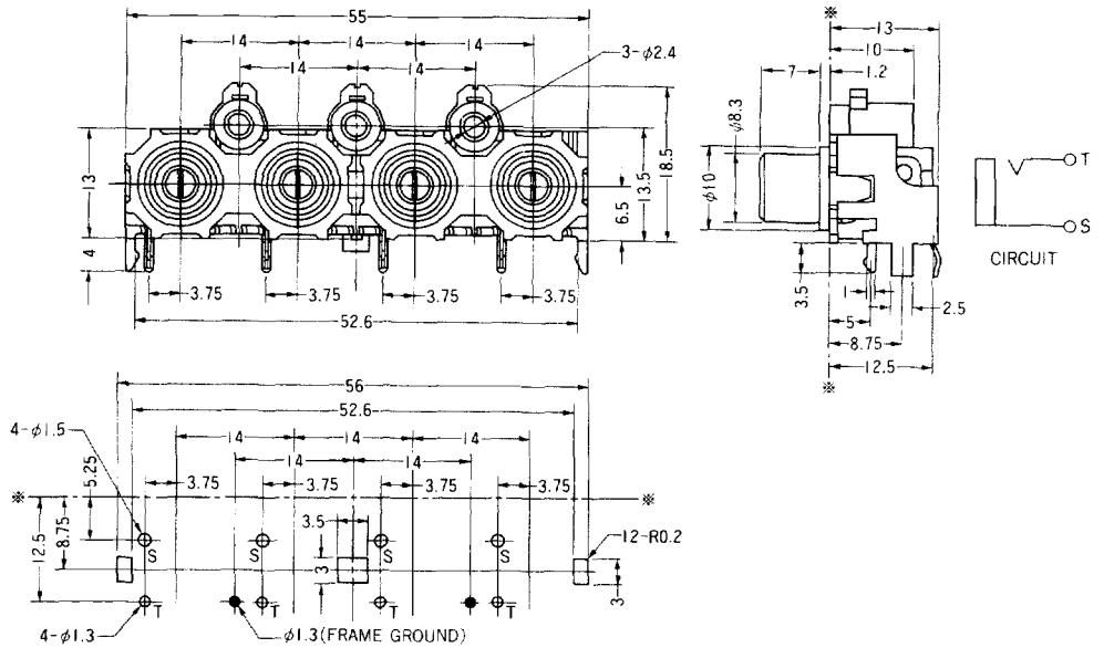
HOLE LAYOUT (PRINTED-SIDE VIEW) PWB t=1.6
