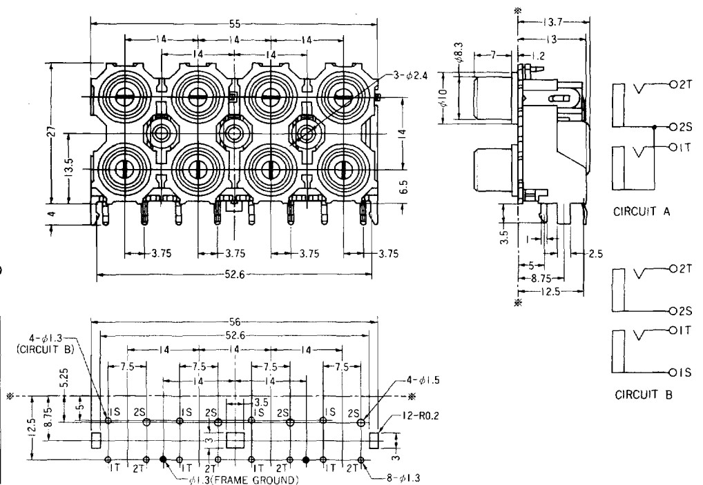
HOLE LAYOUT (PRINTED-SIDE VIEW) PWB t=1.6
