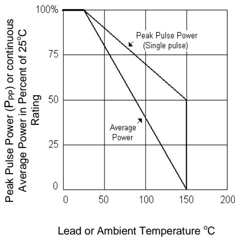
FIGURE 3 Derating Curve
