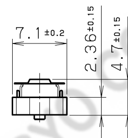
RECEPTACLE LPF-SC200SFYG (N) +
