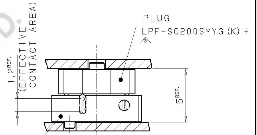
MATED CONDITION (REF.) 嵌合状態図 (参考)
