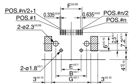
Recommended PCB layout : PAD
