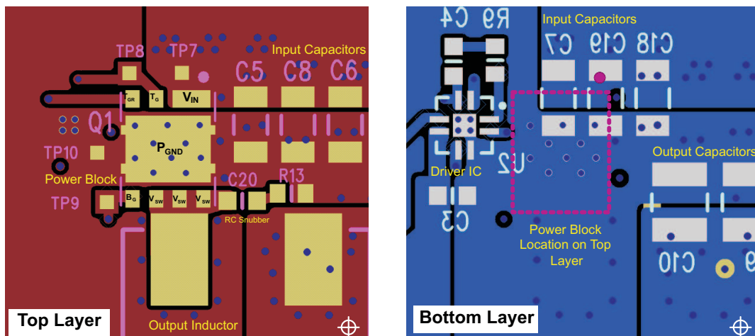
Figure 30. Recommended PCB Layout (Top Down View)
