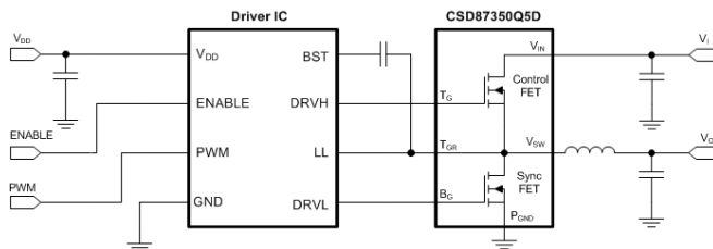
TYPICAL CIRCUIT
