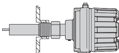
Figure 1 Mounting
