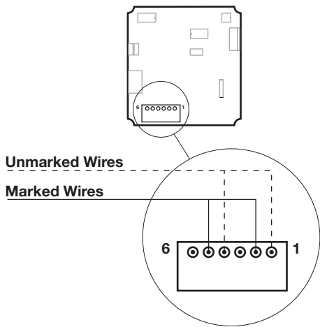
Figure 13 TD2 Probe Connections
