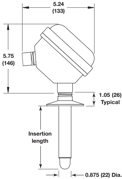
Model TD2 with Hygienic Housing 16-Amp Fitting
