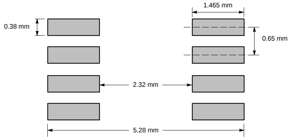
Figure 58. Recommended Footprint
