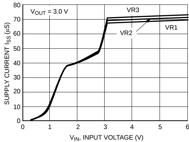
Figure 8. Supply Current vs Input Voltage
