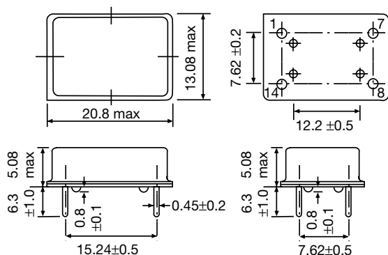
Figure 1) ECS-400X Series – Top, Bottom and Side views
