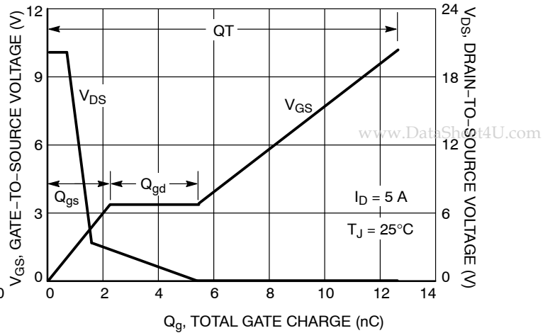
Figure 8. Gate-to-Source and Drain-to-Source Voltage vs. Total Charge
