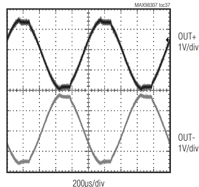
CLIPPING WAVEFORM 10% THD+N
