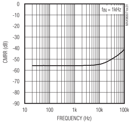
COMMON-MODE REJECTION RATIO vs. FREQUENCY (MAX98307)
