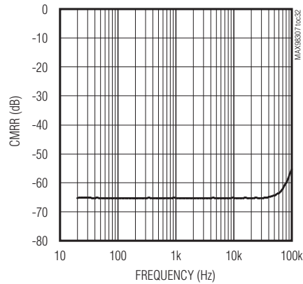
COMMON-MODE REJECTION RATIO vs. FREQUENCY (MAX98308)
