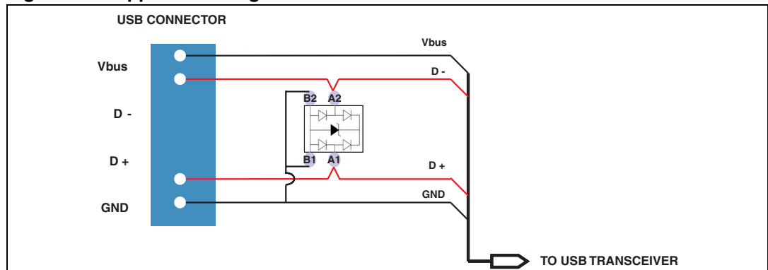
Figure 1. Application diagram
