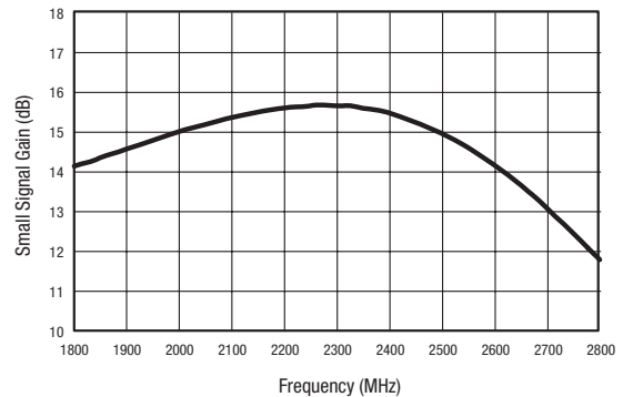
Figure 4. Small Signal Gain vs Frequency, P IN = -20 dBm
