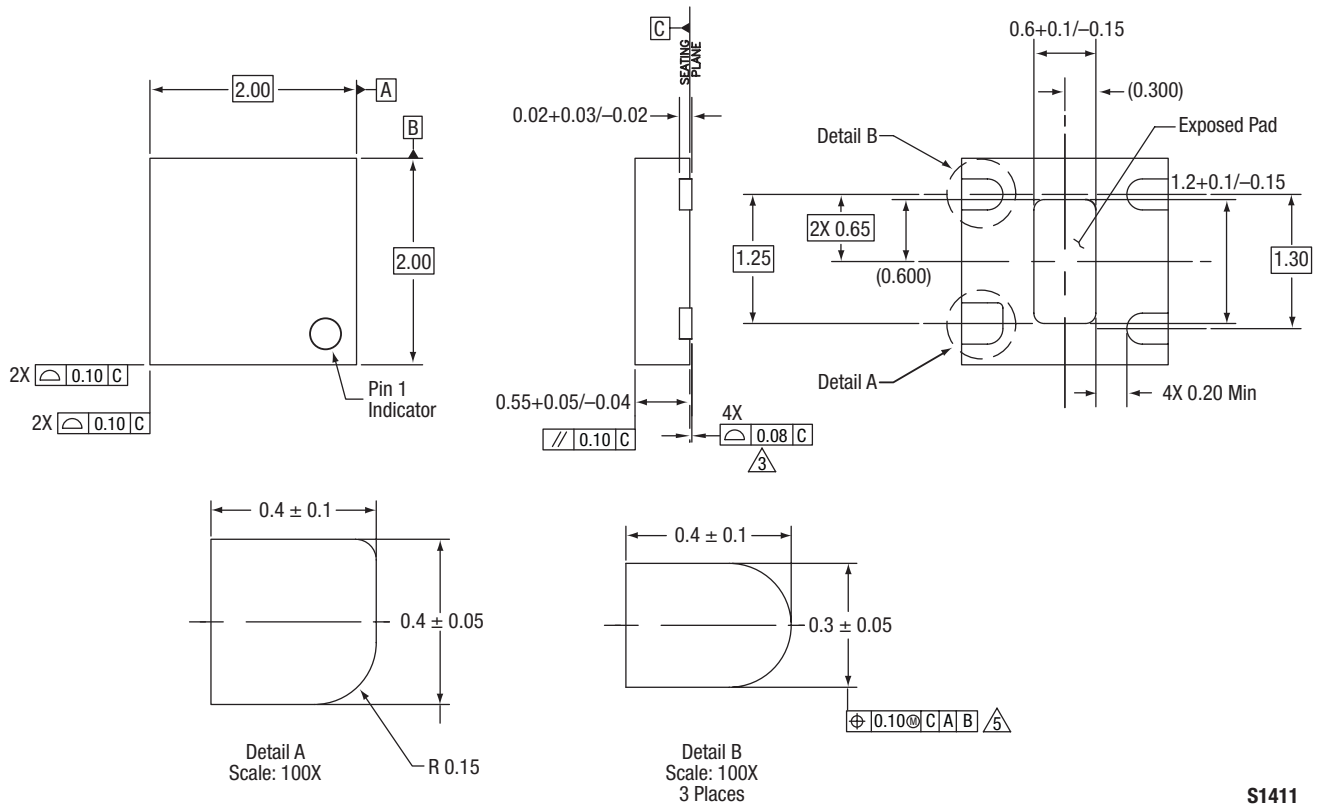
Figure 15. SKY65051-377LF 4-Pin QFN Package Dimensions
