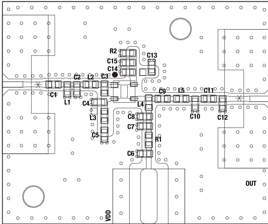
Figure 12. SKY65051-377LF Evaluation Board Assembly Diagram
