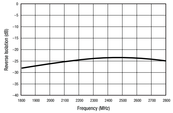
Figure 6. Reverse Isolation vs Frequency, P_{IN} = -20 dBm
