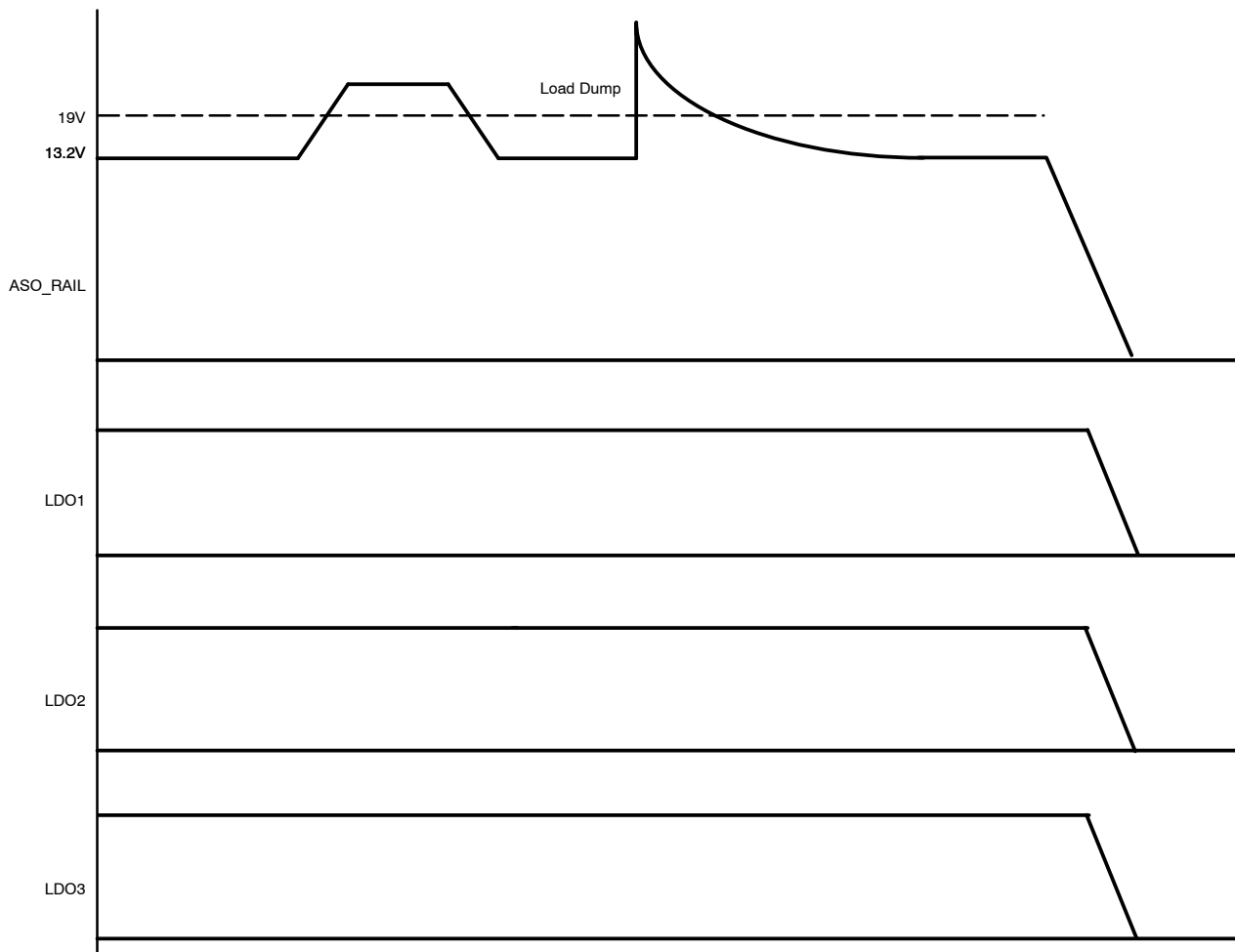
Figure 11. NCV8612 Regulator Output Timing Diagram- VBATT_MON Grounded
