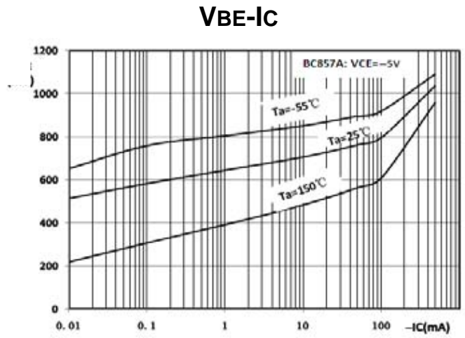
Figure 8. Base-emitter voltage as a function of collector current; typical values
