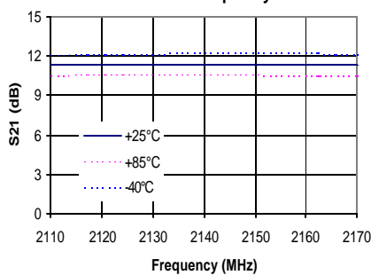
S21 vs. Frequency
