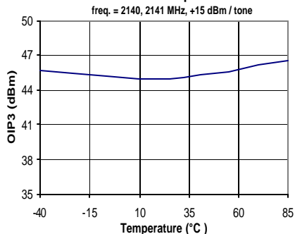
OIP3 vs. Temperature
