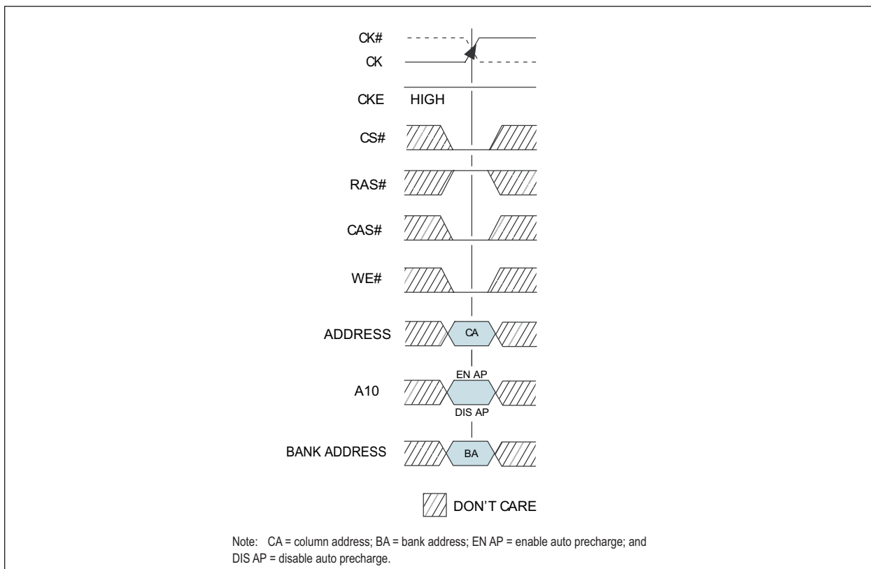
FIGURE 12 – WRITE COMMAND
