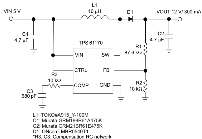
Figure 1. Typical Application
