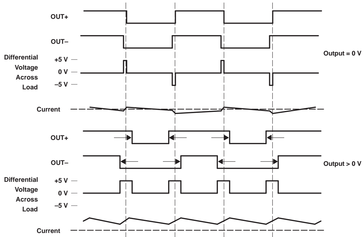
Figure 13. The TPA2000D2 Output Voltage and Current Waveforms Into an Inductive Load
