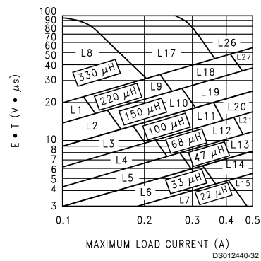
FIGURE 6. LM2597/LM2597HV-ADJ
