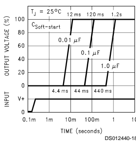
Soft-start Response
