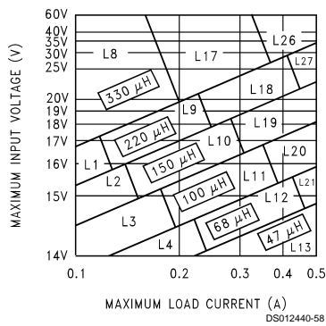
FIGURE 5. LM2597/LM2597HV-12
