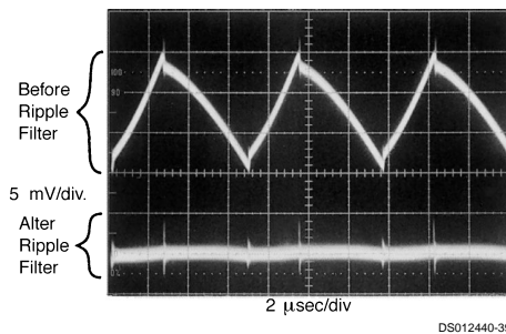
FIGURE 19. Post Ripple Filter Waveform
