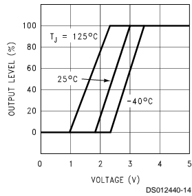
Soft-start
