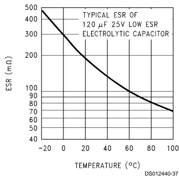
FIGURE 17. Capacitor ESR Change vs Temperature
