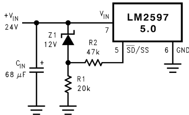
FIGURE 30. Undervoltage Lockout for a Buck Regulator
