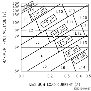
FIGURE 3. LM2597/LM2597HV-3.3
