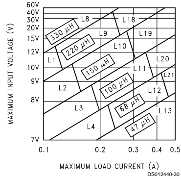
FIGURE 4. LM2597/LM2597HV-5.0
