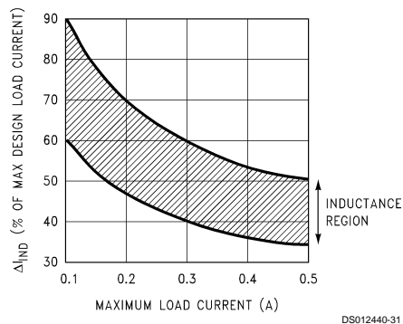
FIGURE 18. ( \Delta I_{LIND} ) Peak-to-Peak Inductor Ripple Current (as a Percentage of the Load Current) vs Load Current
