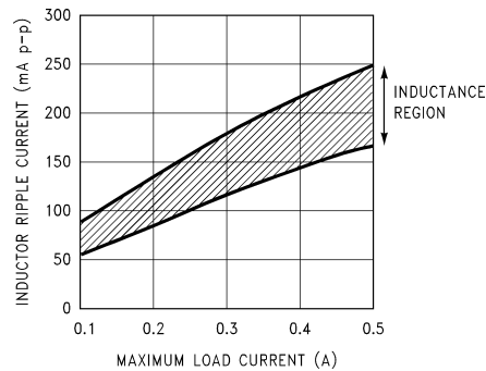
FIGURE 20. Peak-to-Peak Inductor Ripple Current vs Load Current
