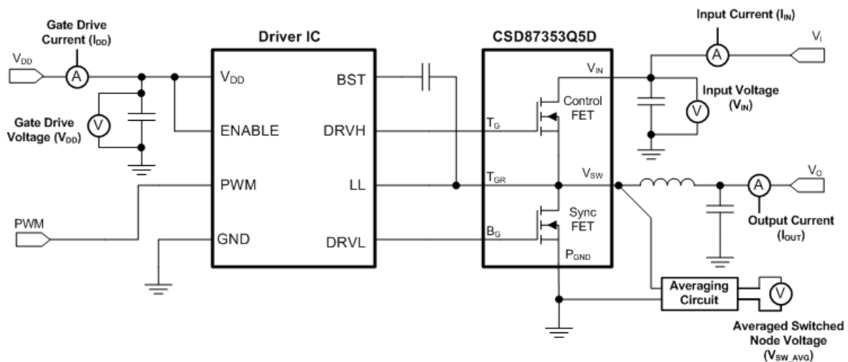
Figure 32. Typical Application
