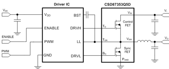
TYPICAL CIRCUIT
