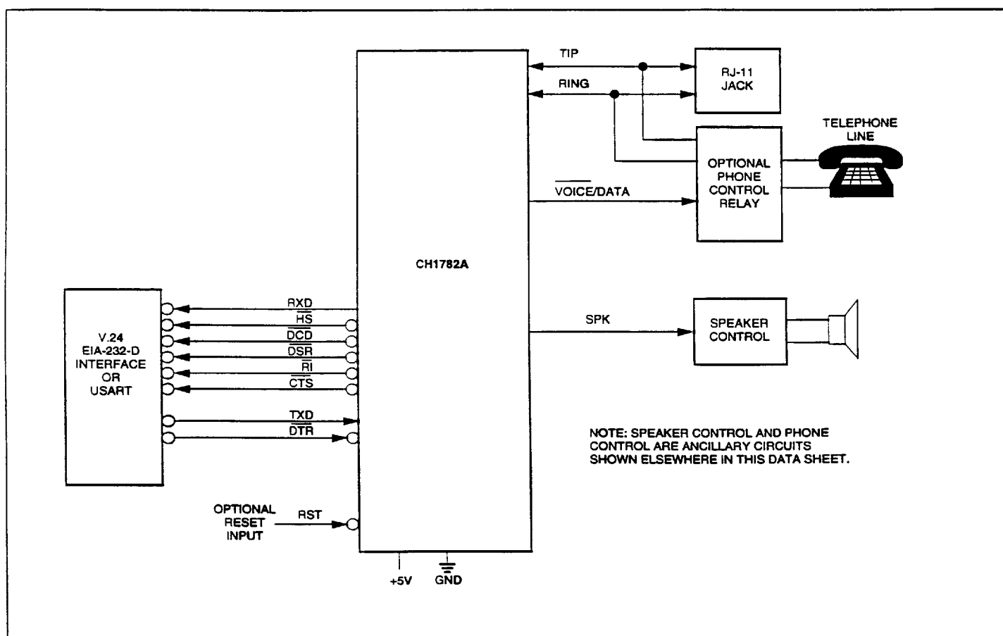
Figure 3a. CH1782A Application Diagram.
