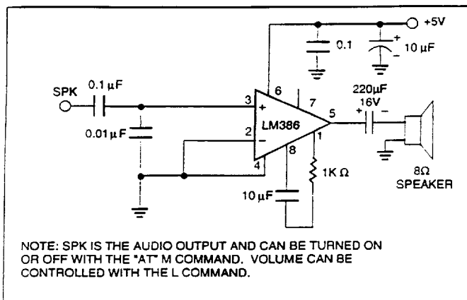
Figure 4. Speaker Control Circuit – optional to allow for call progress monitoring.
