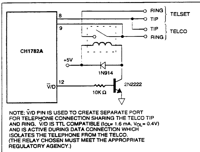
Figure 2. Voice/Data Port Control.
