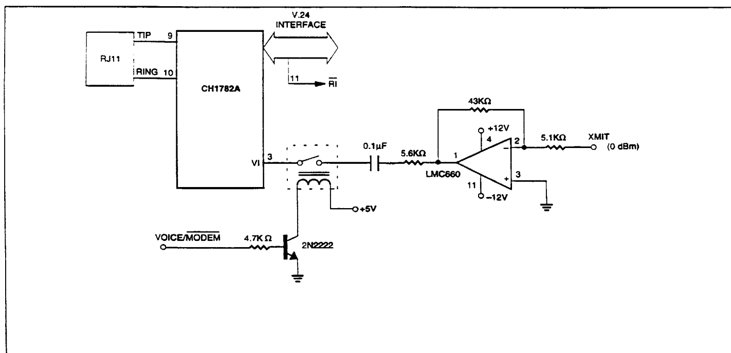
Figure 3b. Using the CH1782A for Voice Application.
