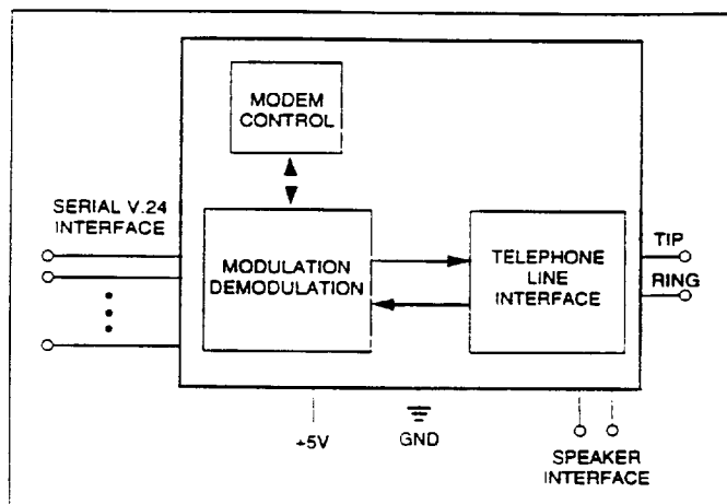
Figure 1. CH1782A Functional Block Diagram.
