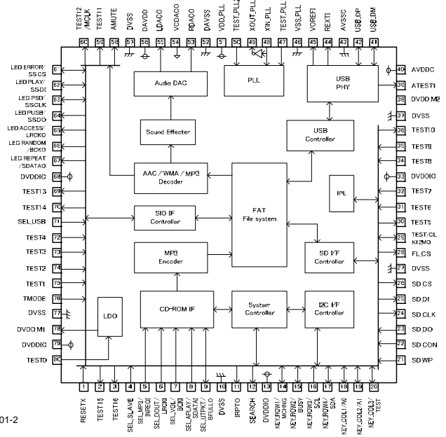
Figure 2. Block diagram
