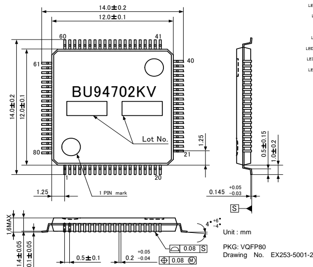
Figure 1. External dimention
