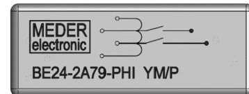
Marking according to EN60062/factory code gem. EN60062/Fertigungsstätte
