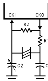
FIGURE 7. Crystal Diagram
