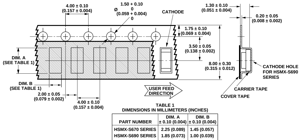
Figure 12. Tape Dimensions HSMx-S670, HSMx-S690.
