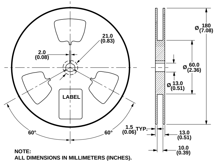
Figure 11. Reel Dimensions.
