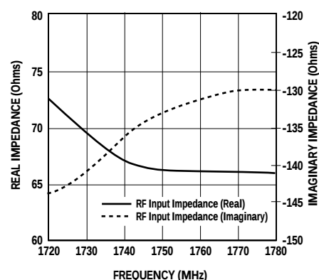
Figure 14. LO Input Impedance (differential) vs. Frequency. [1]
