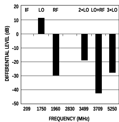
Figure 11. Differential Spur Level at IF pins. [1]
