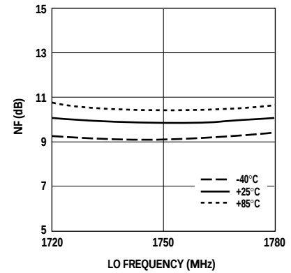
Figure 6. NF vs. LO Frequency.
