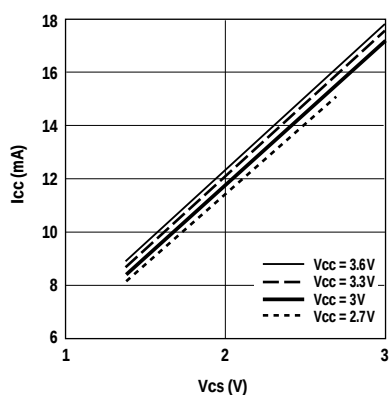
Figure 7A. Icc vs. Vcs.
