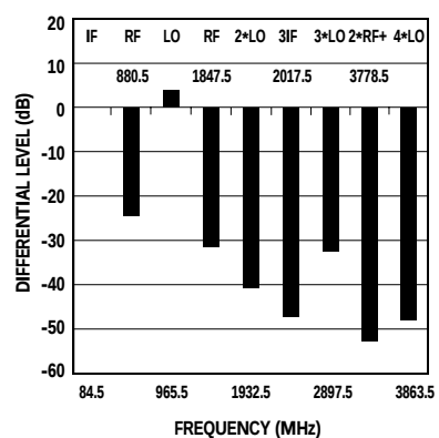
Figure 41. Differential Spur Level at IF pins [1] .
