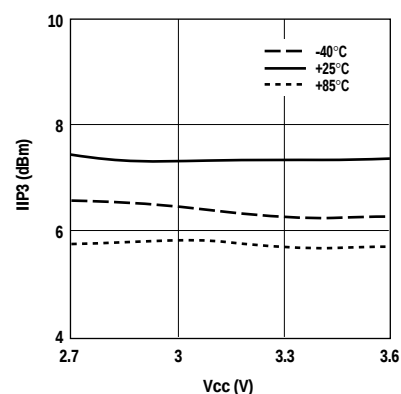
Figure 23. IIP3 vs. Vcc.
