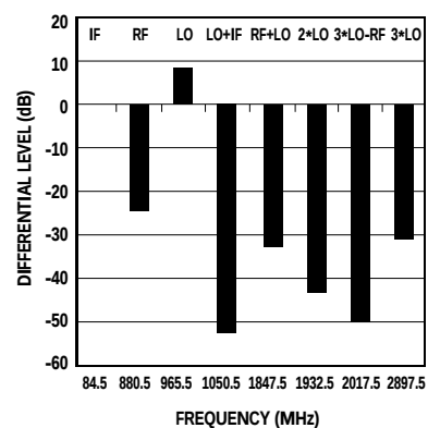
Figure 26. Differential Spur Level at IF pins. [1]
