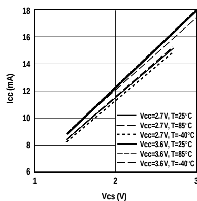
Figure 7B. Icc vs. Vcs.
