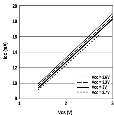
Figure 22A. Icc vs. Vcs.
