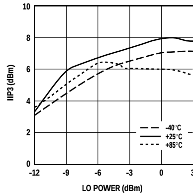
Figure 17. IIP3 vs. LO Power.
