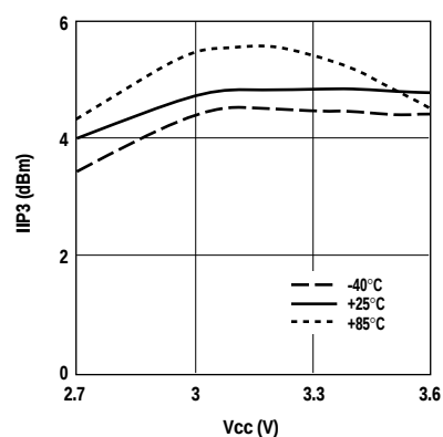
Figure 8. IIP3 vs. Vcc.
