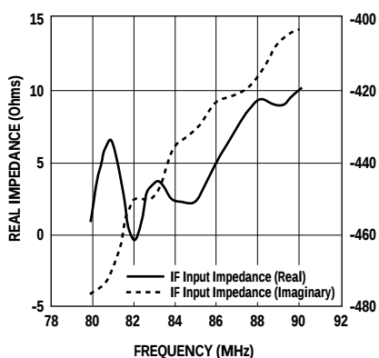
Figure 28. IF Input Impedance (differential) vs. Frequency. [1]
