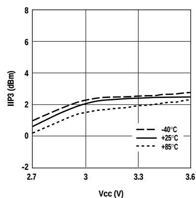
Figure 38. IIP3 vs. Vcc.
