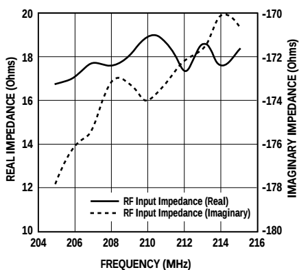
Figure 13. IF Input Impedance (differential) vs. Frequency. [1]
