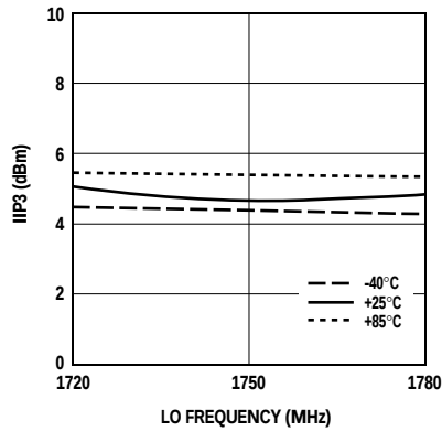
Figure 5. IIP3 vs. LO Frequency.
