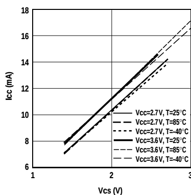
Figure 22B. Icc vs. Vcs.
