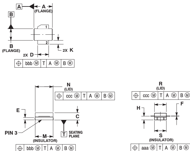
CASE 360C-05 ISSUE D NI-360S MRF9045LSR1
