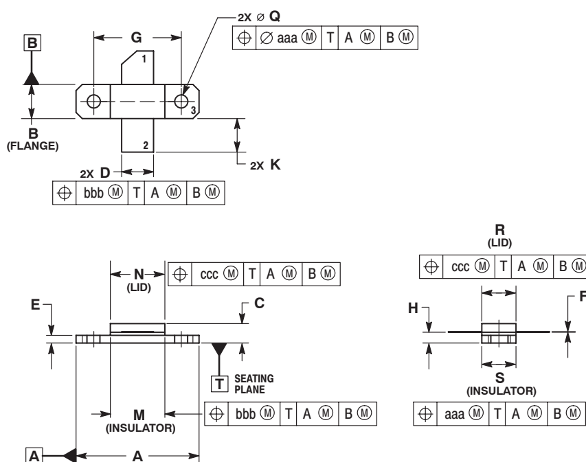
CASE 360B-05 ISSUE F NI-360 MRF9045LR1
