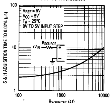
Sample-and-Hold Acquisition Time vs Source Resistance
