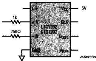
Figure 24a. Overvoltage Protection with Current Limiting Resistors
