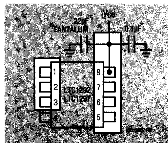
Figure 7. Example Ground Plane for the LTC1292/LTC1297
