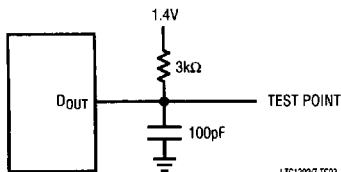
Load Circuit for t_{dD} , t_r and t_f
