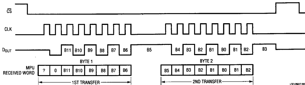
Figure 3. Data Exchange Between LTC1297 and MC68HC11
