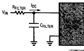
Figure 15. RC Input Filtering
