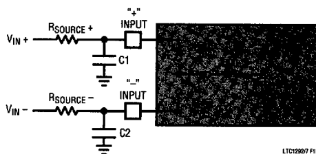
Figure 10b. Analog Input Equivalent Circuit for the LTC1297
