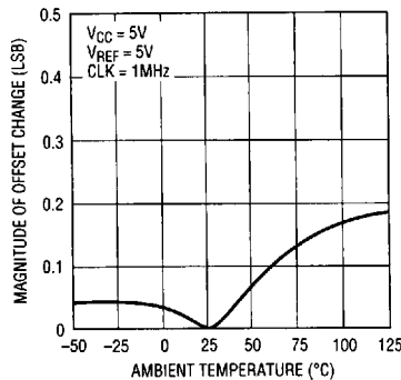
Change in Offset vs Temperature
