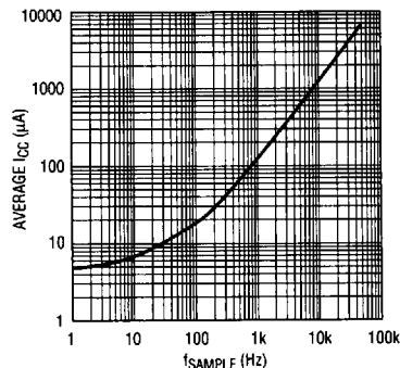
Power Supply Current vs Sampling Frequency
