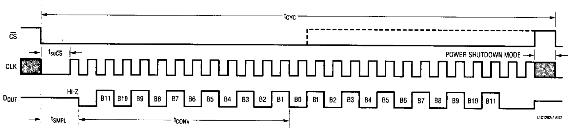
LTC1297 Operating Sequence
