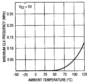
Minimum Clock Rate for 0.1 LSB Error*
