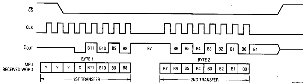
Figure 1. Data Exchange Between LTC1292 and MC68HC11
