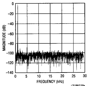
Figure 20a. f_{IN} = 1\text{kHz} , f_S = 58.8\text{kHz} , SNR = 73.0dB
