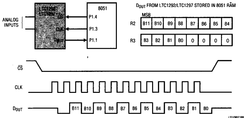
Figure 5. Hardware and Software Interface to Intel 8051 Processor
