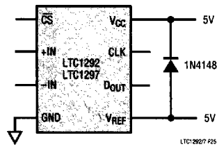
Figure 25. Separate V_{CC} and V_{REF} Supplies
