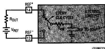
Figure 16. Reference Input Equivalent Circuit
