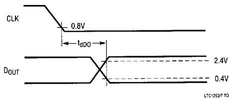
Voltage Waveforms for D_{OUT} Delay Time, t_{dD}
