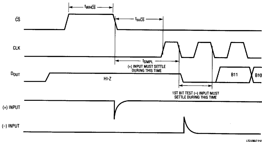
Figure 12. "+" and "-" Input Settling Windows for the LTC1297
