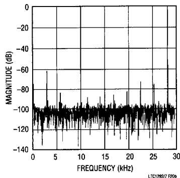
Figure 20b. f_{IN} = 28\text{kHz} , f_S = 58.8\text{kHz} , SNR = 61.5dB
