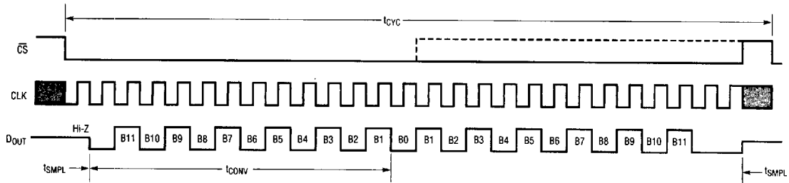
LTC1292 Operating Sequence
