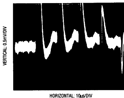
Figure 18. Poor Reference Settling Can Cause A/D Errors
