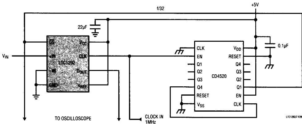
Figure 26. "Quick Look" Circuit for the LTC1292
