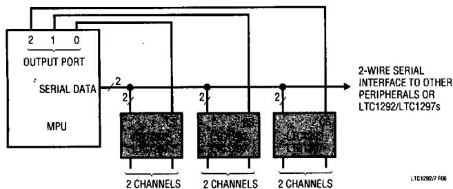
Figure 6. Several LTC1292/LTC1297s Sharing One 2-Wire Serial Interface
