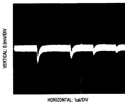
Figure 17. Adequate Reference Settling (LT1027)
