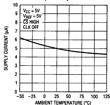
LTC1297 Supply Current (Power Shutdown) vs Temperature
