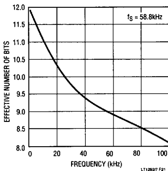
Figure 21. LTC1292 ENOB vs Input Frequency
