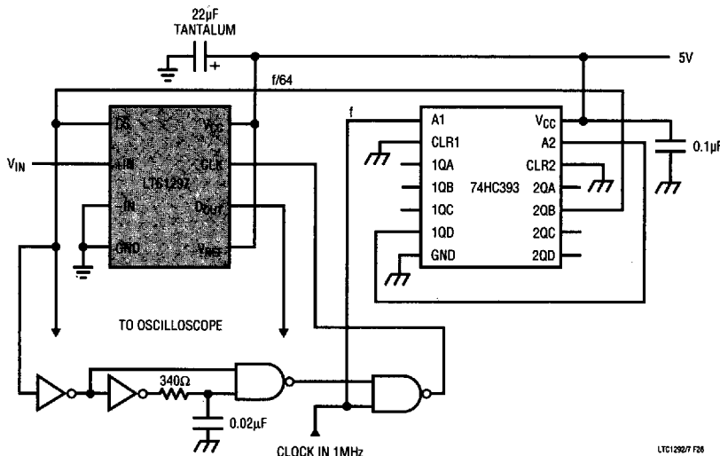
Figure 28. "Quick Look" Circuit for the LTC1297
