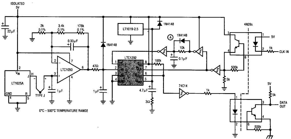
Figure 31. Opto-Isolated Temperature Monitor
